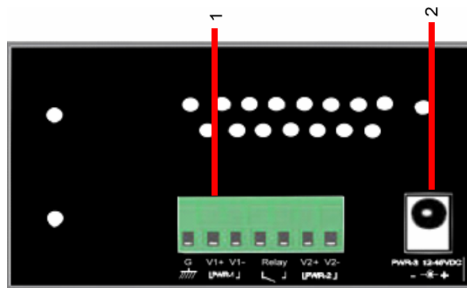
IPS-2042 SERIES power connection
